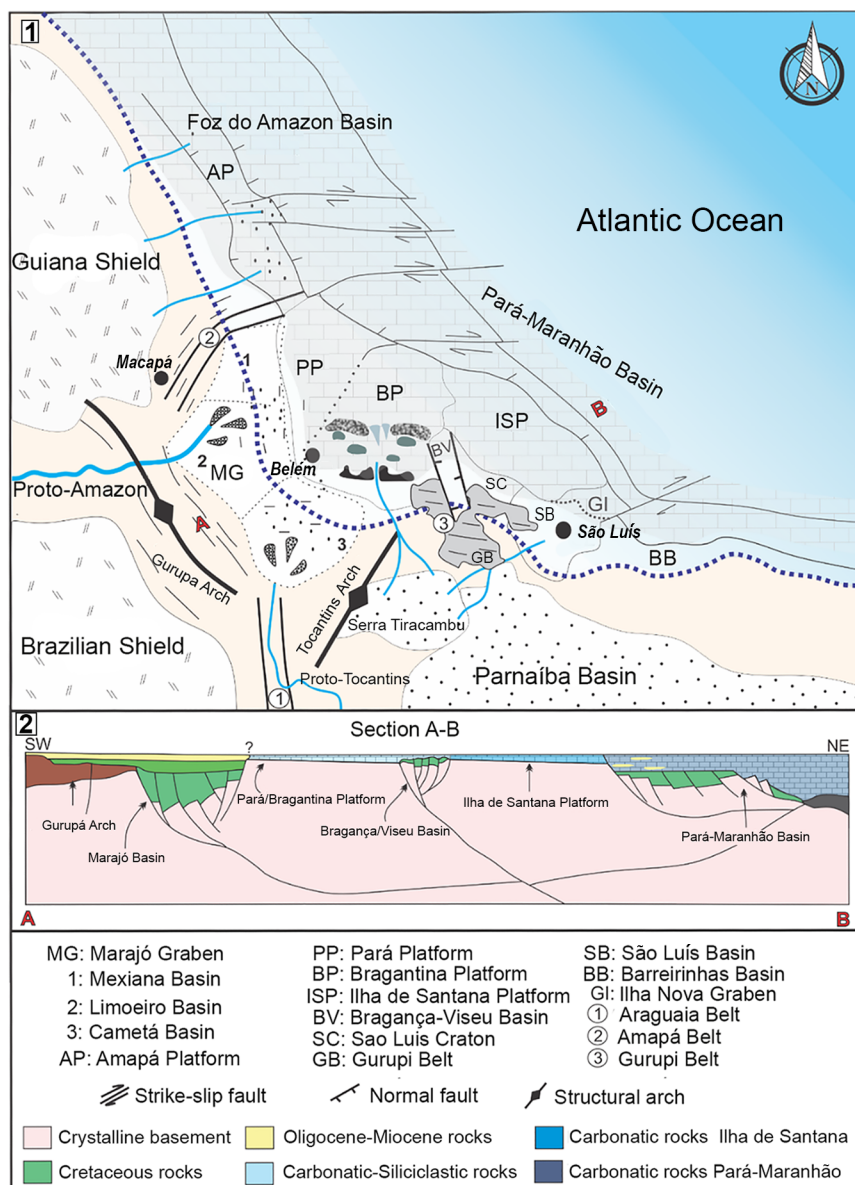
Fig 12. Model of the paleo-Amazon delta during the Oligocene-Miocene in the north coast of Brazil: 1, regional geology and paleo-drainage systems; 2, cross section model (A-B) from the coastal plain to the marine platform.
