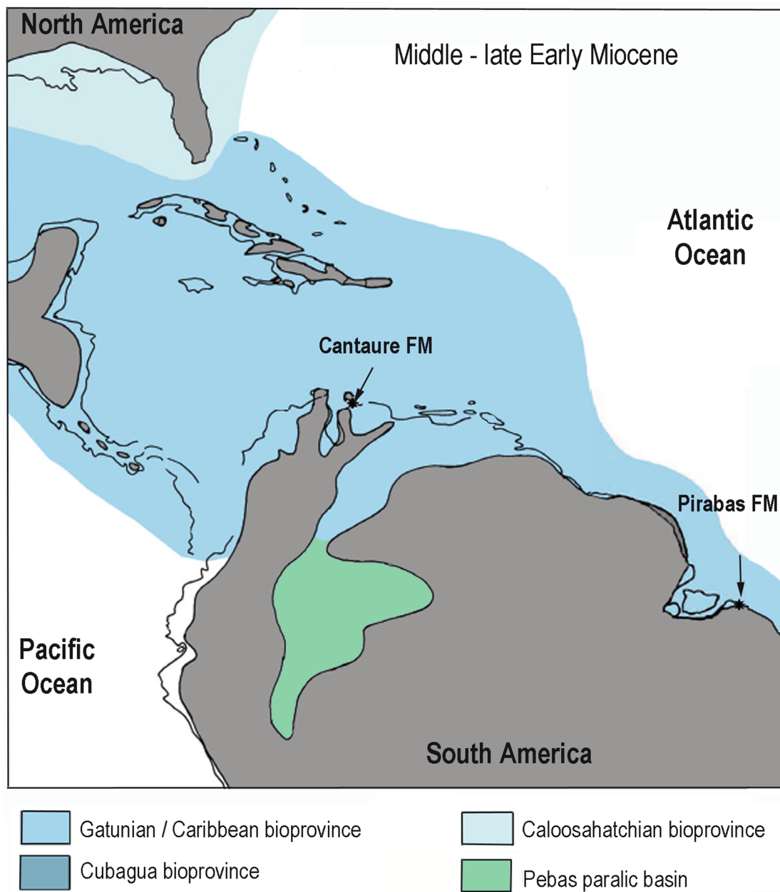
Fig 11. Paleogeographic range of † Carcharhinus ackermannii Santos and Travassos 1960 [23] from both Pirabas and Cantaure formations. Schematic reconstruction modified from [28,142–148]. Reprinted from [28,142] under a CC BY license, with permission from Aguilera O. and Schwarzhans W., original copyright 2016 and 2013 respectively (S3 Appendix).
