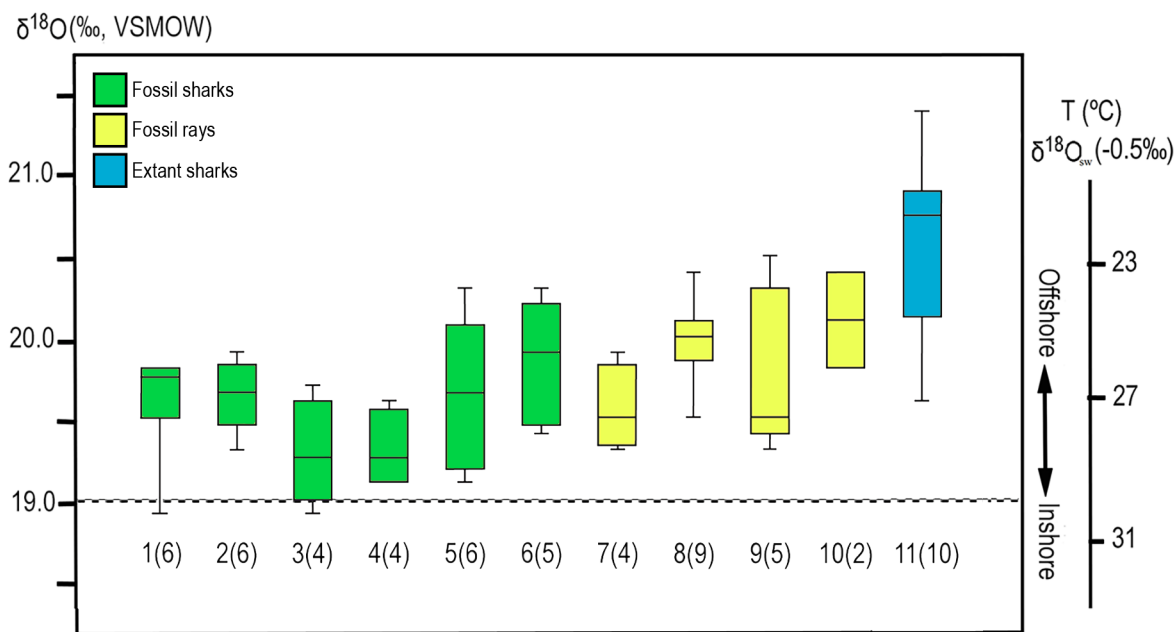
Fig 9. Calculated paleotemperature based on shark and ray tooth \delta^{18}\text{O}_{\text{PO}_4} values from the Pirabas Formation. In green (left): fossil sharks, yellow (center): fossil rays, blue (right): recent sharks. Genus and (n): 1. Galeocerdo mayumbensis (6), 2. Hemipristis serra (6), 3. Carcharhinus sp. (4), 4. Carcharhinus ackermannii (4), 5. Sphyrna sp. (6), 6. Carcharocles chubutensis (5), 7. Aetomylaeus cubensis (4), 8. Aetomylaeus sp. (9), 9. Myliobatoidea (5), 10. Rhinoptera sp. (2), 11. Carcharhinus leucas (9).
