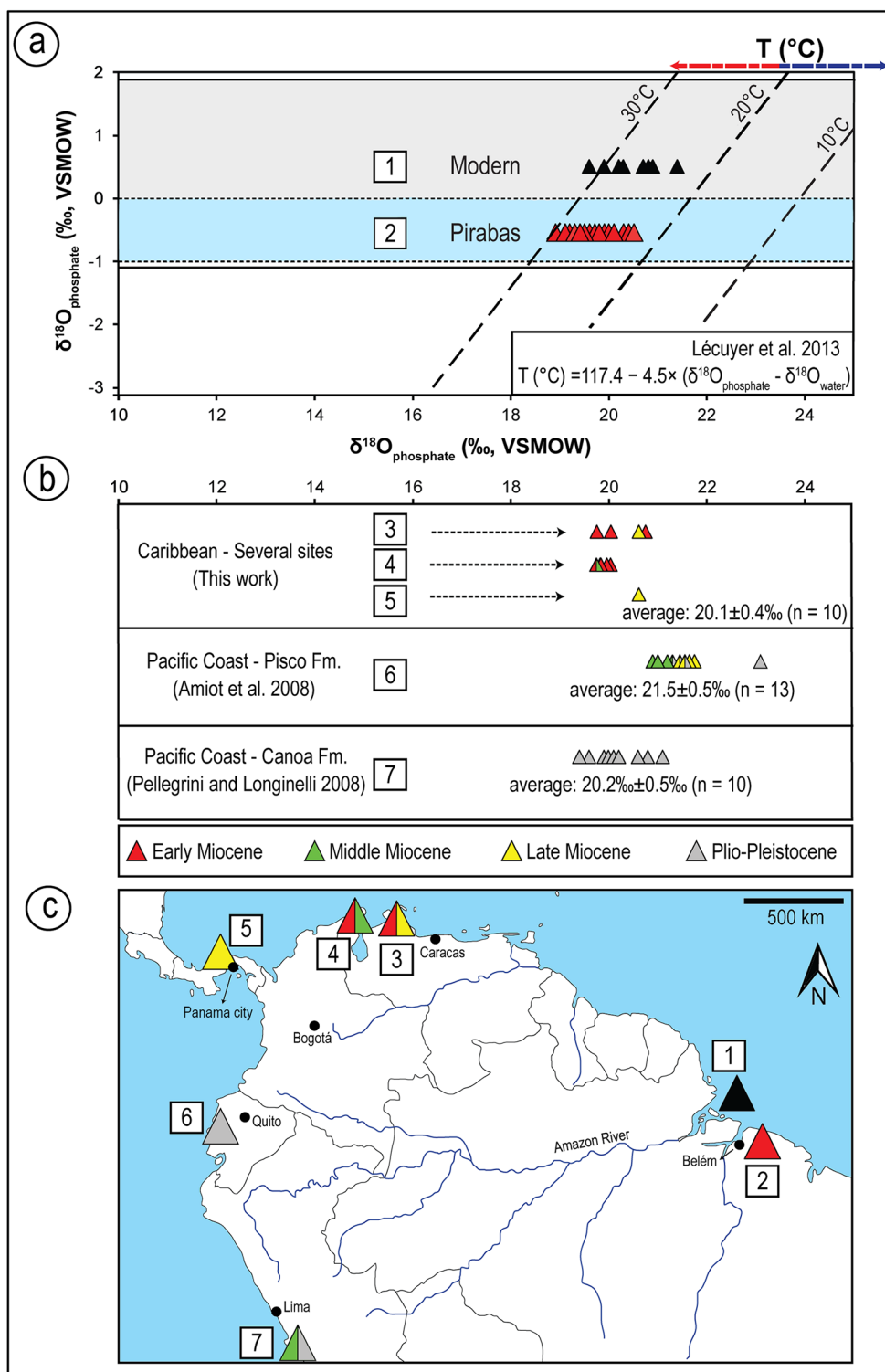
Fig 8. (a) Oxygen isotope composition of phosphate and their relationship as a function of the oxygen isotopic composition of water and temperature. Dashed lines are isotherms calculated from Lécuyer et al. [133]. The blue-shaded area surrounds the isotopic compositions measured for the Pirabean group and represents the variation of early Miocene seawater ( \delta^{18}\text{O}_{\text{w}}: -0.5 \text{‰} , [134]); The gray-shaded zone encircles the isotopic compositions of the Recent group, characterizing the modern fluctuation in the Amazon coastal region ( \delta^{18}\text{O}_{\text{w}}: 0.5 \text{‰} , [135]); (b) Isotopic composition of shark teeth from other fossiliferous deposits of
