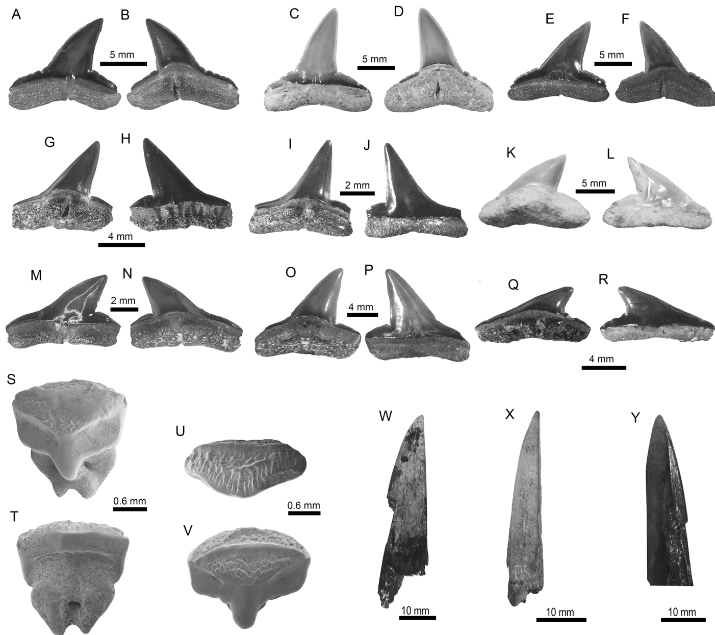
Fig 5. Carcharhiniformes and Rajiformes of the Pirabas Formation. A-F: † Negaprion eurybathrodon (A-B: MPEG-182-V; C-D: MPEG-787-V; E-F: MPEG-1542-V). G-J: † Sphyrna arambourgi (G-H: MPEG-1144-V; I-J: MPEG-1543-V). K-R: † Sphyrna cf. S. laevisissima (K-L: DGM-DNPM-654-P; M-N: MPEG-1838-V; O-P: MPEG-278-V; Q-R: MPEG-811-V). S-V: Rhynchobatus sp. (S-T: MPEG-1951-V; U-V: MPEG-1950-V). W-Y: Pristis sp. (W: MPEG-1873-V; X: MPEG-1874-V; Y: MPEG-1873-V). View: labial (A, C, E, H, J, L-M, P, R, U), lingual (B, D, F-G, I, K, N-O, Q), posterior-occlusal (S), anterior-basal (T), occlusal (V), dorsal (W-Y).
